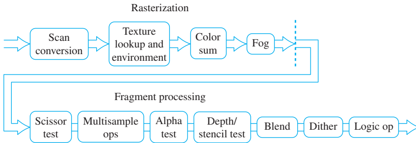
Figure 6.1 Rasterization pipeline.
