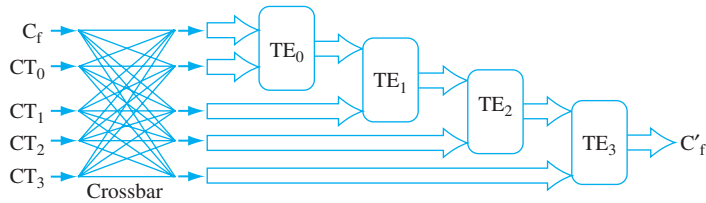
Figure 5.11 Multitexture texturebar environments. Four texture units are shown; however, the number of units available depends on the implementation. The input fragment color is successively combined with each texture according to the state of the corresponding texture environment, and the resulting fragment color passed as input to the next texture unit in the pipeline.
